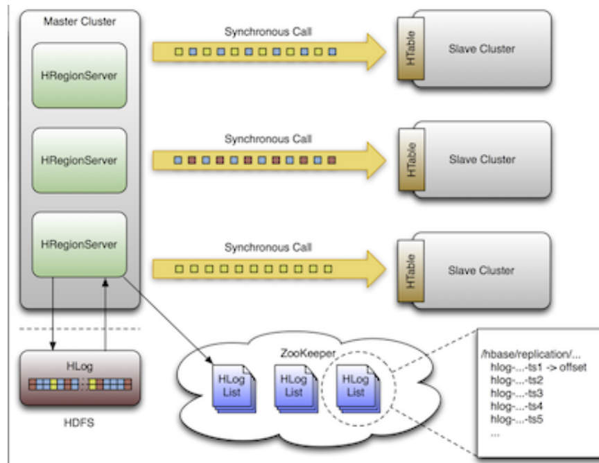
Figure 4.2. HBase Replication Architecture Overview
